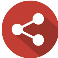
Social Bookmarking
